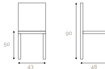
Chair art. 161/S
