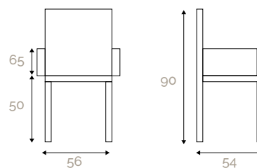
Armchair art. 162/C
