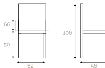
Armchair art. 174/C
