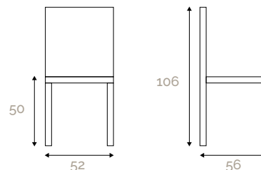
Chair art. 174/S
